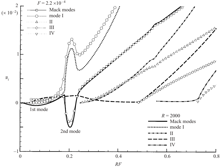
FIGURE 10. The distribution of the growth rates of boundary-layer wave modes as a function of RF obtained by the LST.
