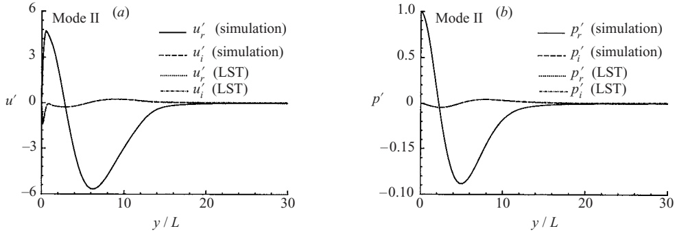
FIGURE 25. Comparison of the wave structure of mode II obtained by the LST and by numerical simulation for grid station located at R = 1874.46 for the case of imposed mode II at inlet with RF = 0.3552 ( F = 2.2 \times 10^{-4} ).
